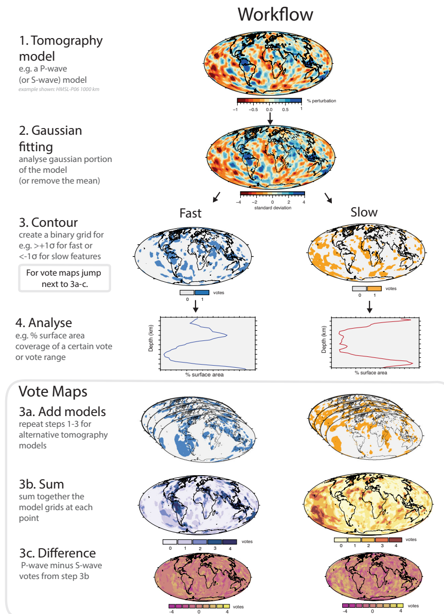
Fig. 3 Workflow used in this paper. Step 1: select tomography model. Step 2: a gaussian fitting procedure is applied (see Methods). Step 3: a contour metric is chosen e.g. fast ( >+1\sigma from the mean), and slow ( <-1\sigma from the mean) and binary grids are created. Step 4: surface area coverage of the contour is extracted across the lower mantle. For the vote map methodology additional steps are applied between Steps 3 and 4. Step 3a: binary grids from additional tomography models are created as per Steps 1-3. Step 3b: at each grid point the constituent models (here 4 models) are summed. Step 3c: difference vote maps can be generated, for example by subtracting the S-wave votes from the P-wave votes.
